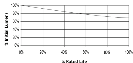
Lumen Maintenance
