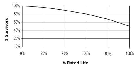
Lamp Mortality
